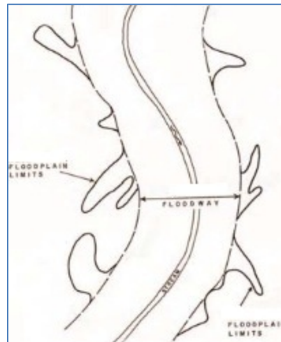
Figure 2 – Shallow areas that do not effectively convey flood waters not included in the floodway. (Source: modified from MN DNR – Technical Report 6 1972)
