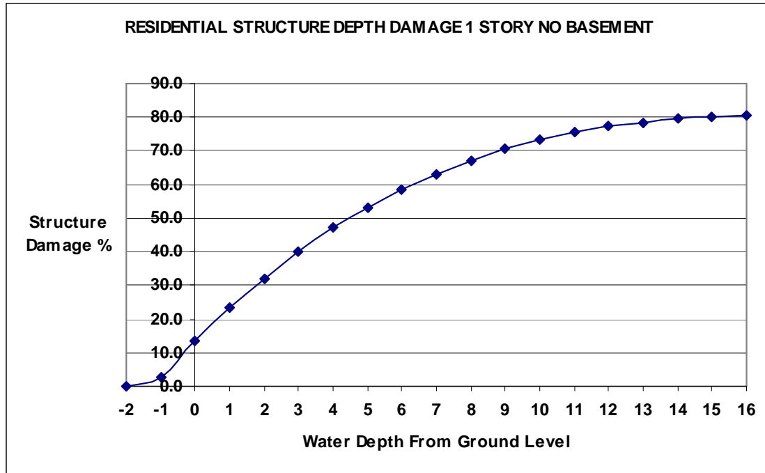
Figure 3 – Flood Depth-Damage Curve for a Single-Story Residential Structure with No Basement at Ground Level. (Source: U.S. Army Corps of Engineers Floodplain Inventory Tool (CEFIT))
