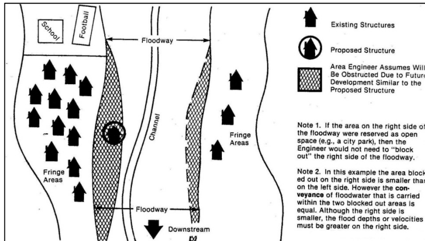
Figure 5 – Using Equal Degree of Encroachment principles in evaluating development proposals. (Source: The Floodway: A Guide for Community Permit Officials (FEMA, 1978))
