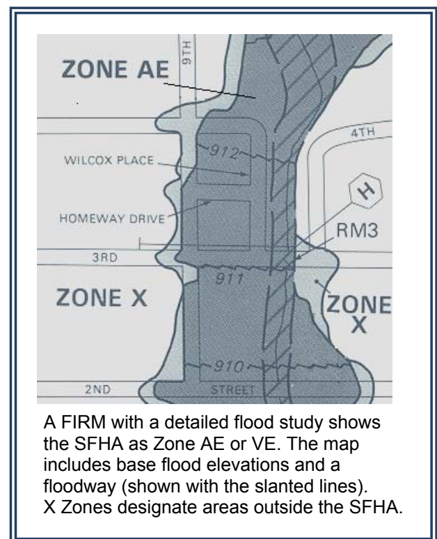
Figure 410-1. FIRM terminology.
